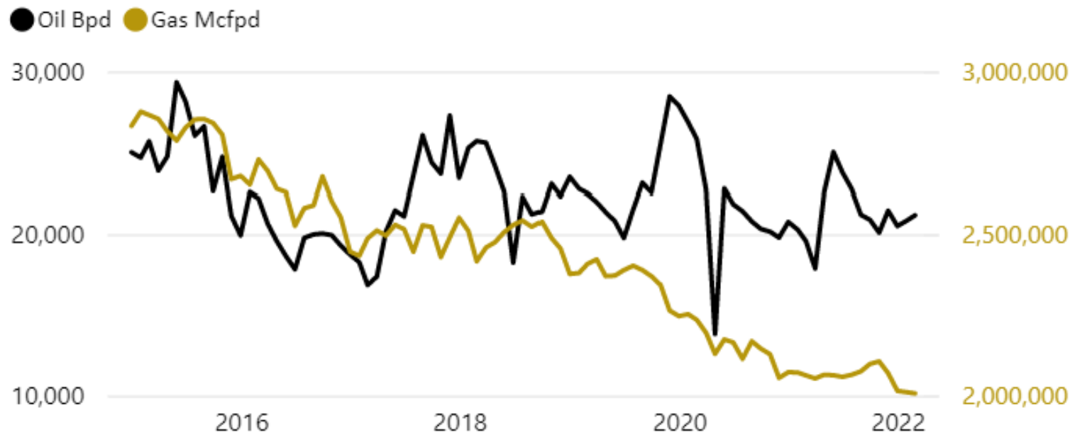
San Juan Basin Oil and Gas Production
