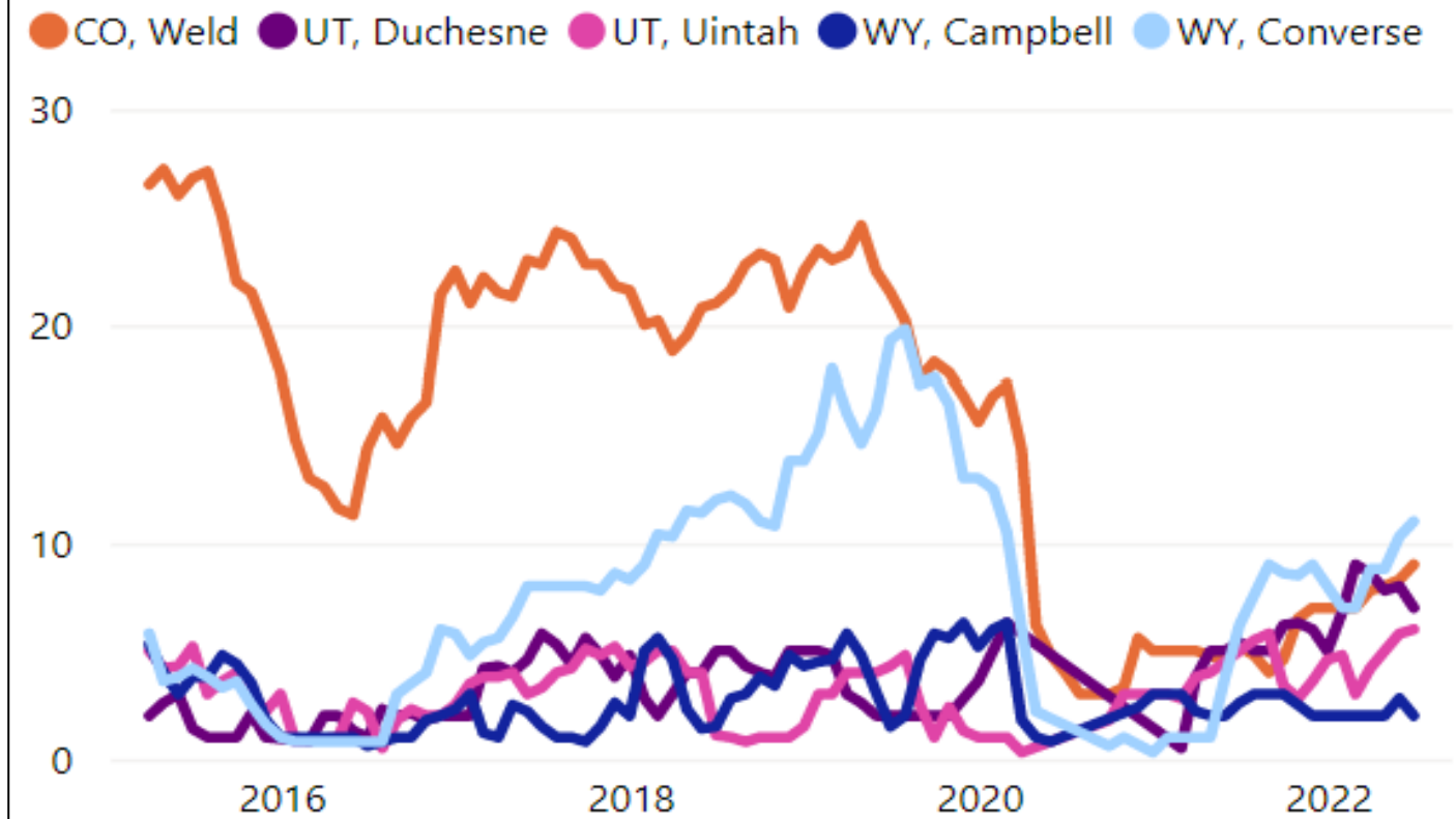
Count Rigs Drilling by Month
